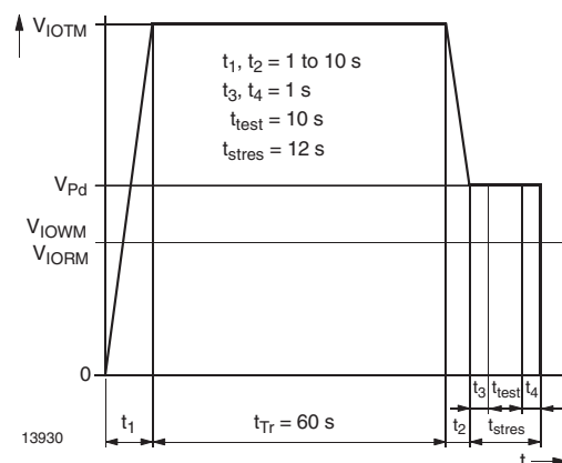
Figure 5. Test pulse diagram for sample test according to DIN EN 60747-5-2(VDE0884)/ DIN EN 60747-5; IEC60747
