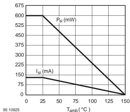
Figure 4. Derating diagram
