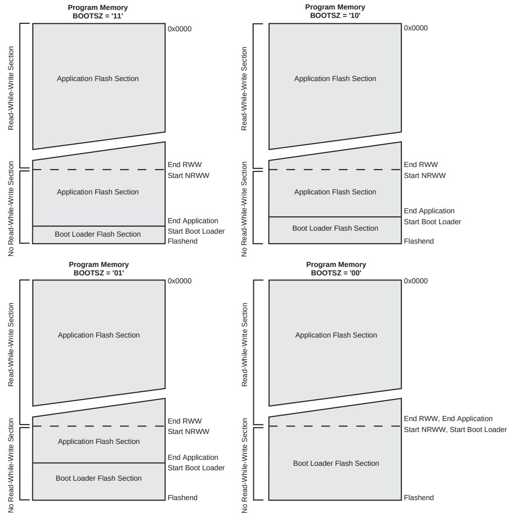
Figure 26-2. Memory Sections
